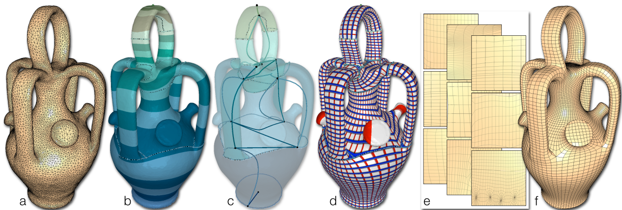
Fig. 1. For an input polygonal model (a), our interactive quadrangulation framework is driven by a user-defined scalar field (b), that guides a Reeb atlas segmentation of the model into a coarse quadrangulation capturing the dominant features of the shape (c) and allows control of the extraordinary vertices. Since the charts of the Reeb atlas have a guaranteed generic topology, they can be efficiently parameterized to the unit square (d). Designing connectivity textures of the unit square (e) enables an easy yet flexible quad-only meshing of the charts, providing a fine-grain control for the explicit capture of the high-frequency geometric details, while maintaining interactive rates of editing operations.
