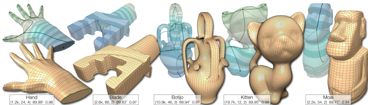
Fig. 12. Various examples of user designed quad meshes generated with our framework accompanied by quality statistics related to the vertices (vertex count, extraordinary vertex count and the max difference from the ideal valence), the average mesh angle and scaled Jacobian.
