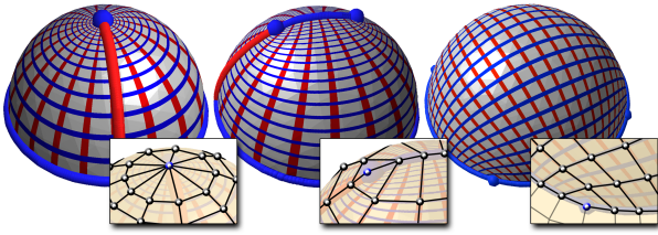
Fig. 6. Fractional poles: a polar vertex (left) split into 2 half-poles (valence 2, middle) and 4 quarter-poles (valence 3, right).
