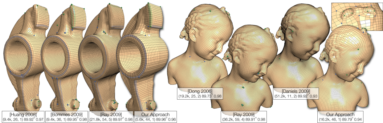
Fig. 14. The comparison of our technique against quad meshes from multiple algorithms illustrates our improved control of extraordinary vertices, i.e. location and valence, as well as element alignment, while producing quality output models for the Rocker Arm and Bimba models. Extraordinary vertices with a valence greater or less than four are respectively reported with blue and green spheres. Shaded quad-strips highlight the twisting occurring with previous approaches along sharp features (blue) or between extraordinary vertices (green).
