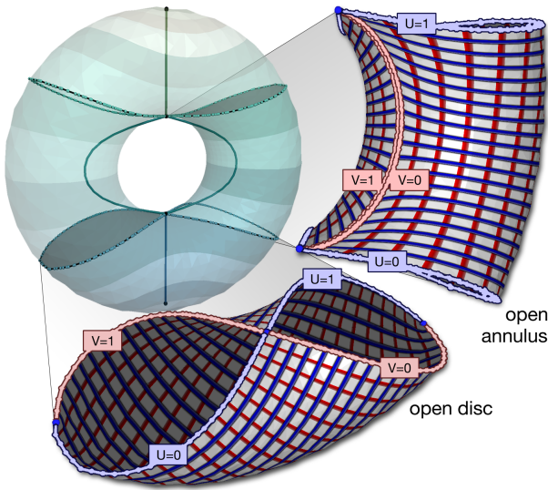
Fig. 3. Our parameterization strategy maps the boundaries of the Reeb chart (homeomorphic to an open annulus or open disc) to the unit square by defining UV Dirichlet boundary conditions within the Laplace system. Open annuli are cut into discs by a streamline guided by the scalar field gradient.
