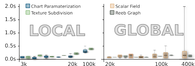
Fig. 13. Boxplot response timings of our system computations, measured in seconds as a function of the number of input triangles.
