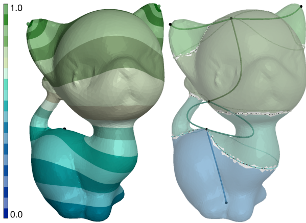
Fig. 2. The harmonic scalar field f is drafted by the user, modifying the automatically suggested extrema. Reeb charts, constructed from the arcs of the Reeb graph, segment the model into multiple regions with known topology: annuli and discs.
