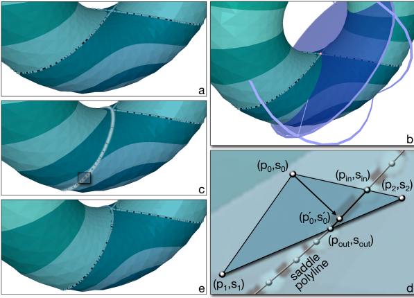
Fig. 4. Reorienting a saddle contour: the original levelset curve (a) is modified through the critical contour widget (b) where the mesh-plane intersection describes the new contour geometry (c). Saddle triangles are constrained (d) to ensure the scalar field respects the critical contours (e).
