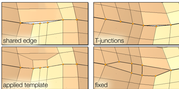
Fig. 10. T-junctions are resolved by the stitching process: inserting new quads where multiple T-junctions share a common edge (a), or performing mesh surgery along the path between two nearby triangles and inserting quads along the cut (b).
