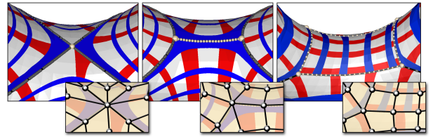
Fig. 7. Fractional saddles: a saddle vertex (valence 8, left) split into 2 half-saddles (valence 6, middle) and 4 quarter-saddles (valence 5, right).
