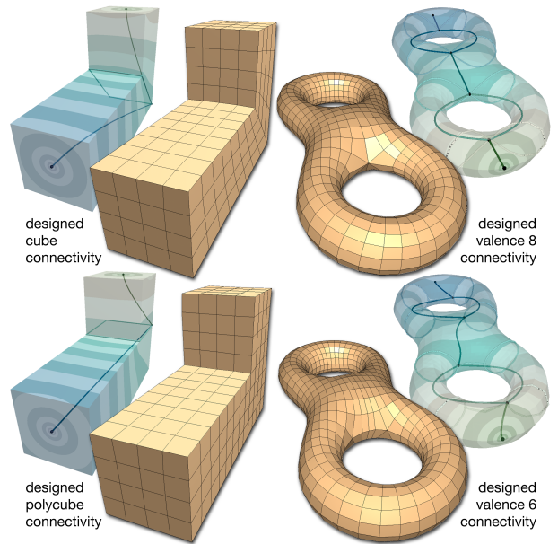
Fig. 11. Our multi-level approach to quad design (global segmentation and local design) is flexible, making it possible to design different quad connectivities and extraordinary vertex types over the same model. Note that a Reeb graph with a single arc is divided (left), describing two Reeb charts with disc topology.
