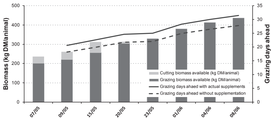
Figure 2. Evolution of grass available and grazing days ahead.
