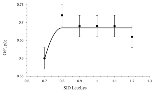
Figure 3. Curvilinear plateau model estimated the optimum standardized ileal digestible (SID) Leu:Lys at 0.80 \pm 0.01 ( Y = 0.685 - 8.8 \times (0.80 - x)^2 ). The broken-line model could not be fitted to the G:F data. Data points (·) represent least squares mean \pm SEM for each dietary treatment ( n = 16 pigs per treatment).
