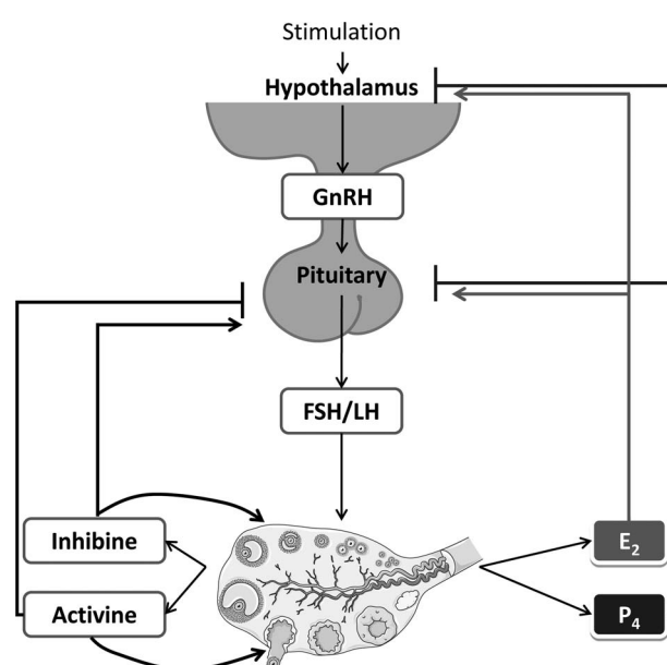
Figure 1 Schematic representation of the hormonal regulation of ovarian activity. E2 = estradiol, P4 progesterone → stimulation; ⊥ inhibition.
