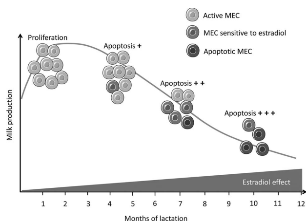
Figure 6 General diagram showing the action of estradiol on ovarian mammary epithelial cells (MECs) during lactation in not pregnant dairy cows. After the peak of lactation, the number of MEC decreases and increases sensitivity to estradiol. Estradiol acts then on MEC to induce and accelerate the process of apoptosis, which increases the loss of MEC and lower milk production. The increasing effect of estradiol during lactation on MEC and milk production is represented by the red triangle.
