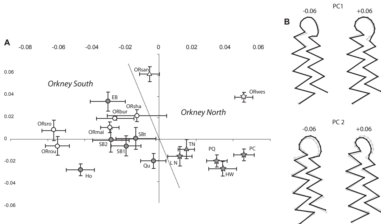
Figure 6. Molar shape variation in modern and ancient Microtus arvalis samples from Orkney. (A) Scatter plot of the two first principal components of the morphometric analysis. The modern samples are represented by empty symbols whereas the ancient samples are shown by gray-filled circles. The dotted line separates northern from southern populations. (B) Molar shape change associated with PC1 and 2 is depicted by a wireframe graph connecting the landmarks and semilandmarks. The gray wireframe represents the mean shape and the black wireframes indicate the shape change of the PC score by 0.6 units in the positive and negative directions.
