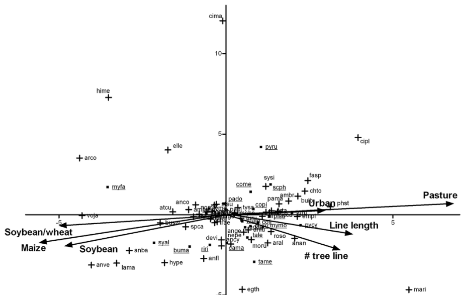
Figure 3 Ordination plot for CCA at facet scale. Only variables with the highest interset correlations are drawn. Species are identified using four letter keys (see Additional file 1: Table S1). Species with underlined keys and square symbols are exotic to the Pampas. Ordination explains 2.8% of total variance.
