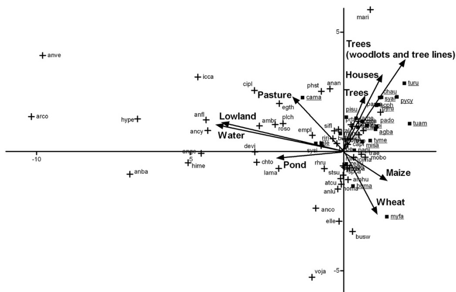
Figure 2 Ordination plot for CCA at local scale. Only variables with the highest interset correlations are drawn. Species are identified using four letter keys (see Additional file 1: Table S1). Species with underlined keys and square symbols are exotic to the Pampas. Ordination explains 5% of total variance.
