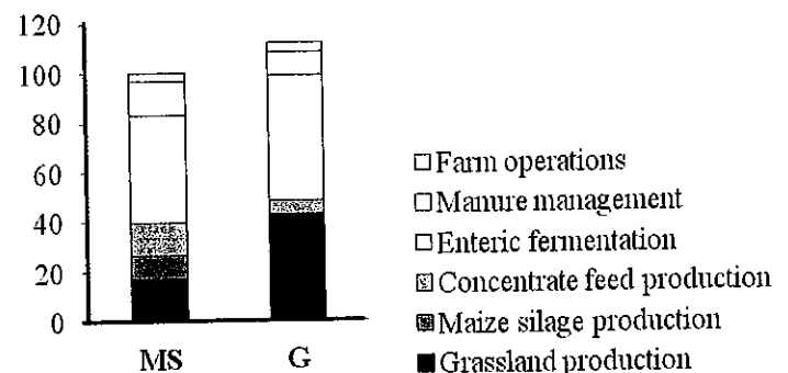
Figure 1 Contribution (in %) of main processes to GHG emissions per kg FPCM of dairy systems based on maize silage and grass (MS) or on grassland only (G) (MS represents 100%, G is relative to MS)
