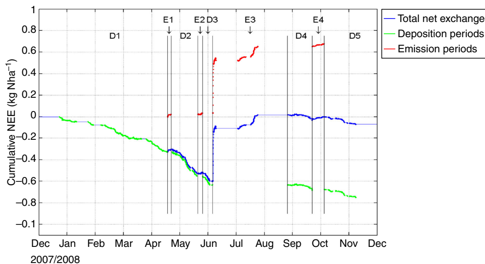
Fig. 11. Cumulative net \Sigma\text{N}_r exchange during the entire observation period from December 2007 to November 2008. The red line indicates the cumulative net \Sigma\text{N}_r loss to the atmosphere during net emission periods, the green line indicates the cumulative net \Sigma\text{N}_r gain of the plant–soil system during net deposition periods, and the blue line represents the cumulative total net \Sigma\text{N}_r exchange. Periods D1–D5 and E1–E4 correspond to naming in Table 1.
