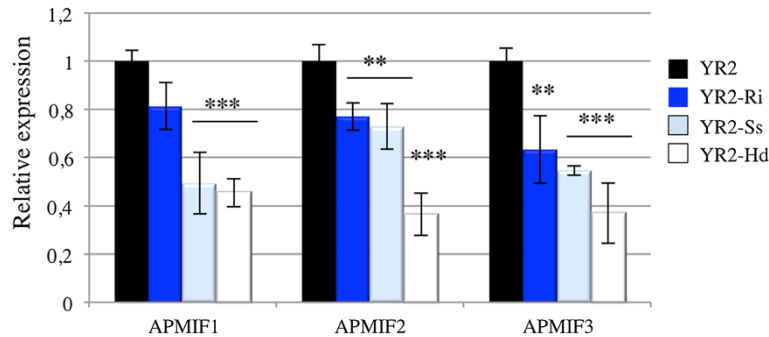
Figure 4 Comparison of ApMIFs expression in YR2 aphids associated with R. insecticola (YR2-Ri), S. symbiotica (YR2-Ss) or H. defensa (YR2-Hd). Expression has been normalized to EF1 expression and to expression in control aphids (black). Each bar represents the mean expression \pm SD obtained from three independent experiments. Significant differences as compared with control are indicated by stars (Anova on row data: ***: p < 0.0002 ; **: p < 0.002 ).
