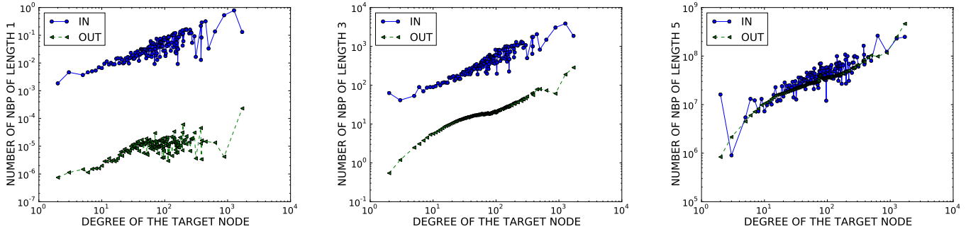
Fig. 2. Average number of NBP of length 1, 3 and 5 (from left to right) as a function of the degree of the target node between a source and a target node in the category “Graph theory” (in) and a source node within the category and target node outside the category (out).
