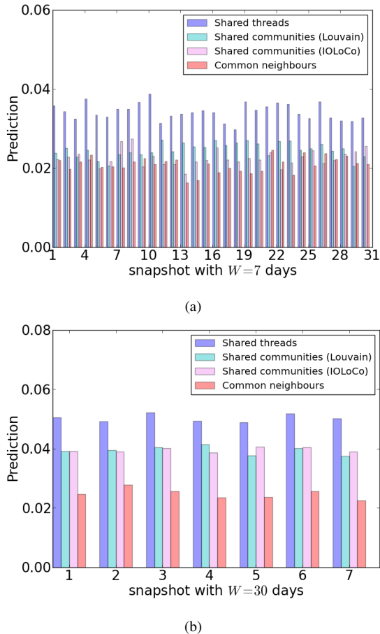
Fig. 6: Prediction results for different methods on Debian Dataset with different time windows: (a) W = 7 days. (b) W = 30 days. Here the result is obtained by running each method 100 times.
