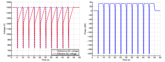
(a) DC voltage reference and effective DC voltage
