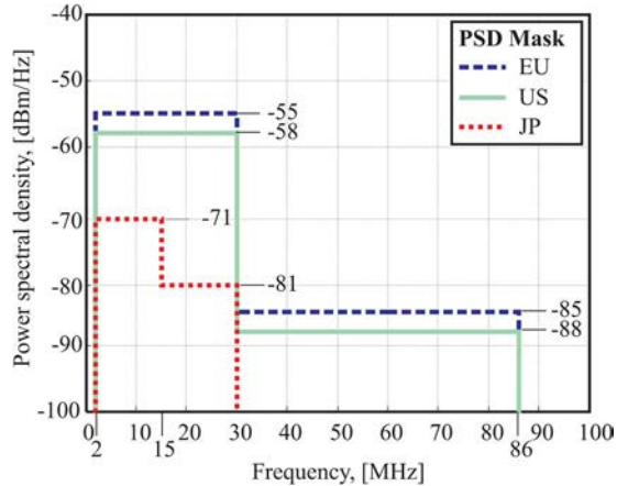
Fig. 6. Transmit PSD masks. Note, the EU limit above 30 MHz is subject to pending regulations.
