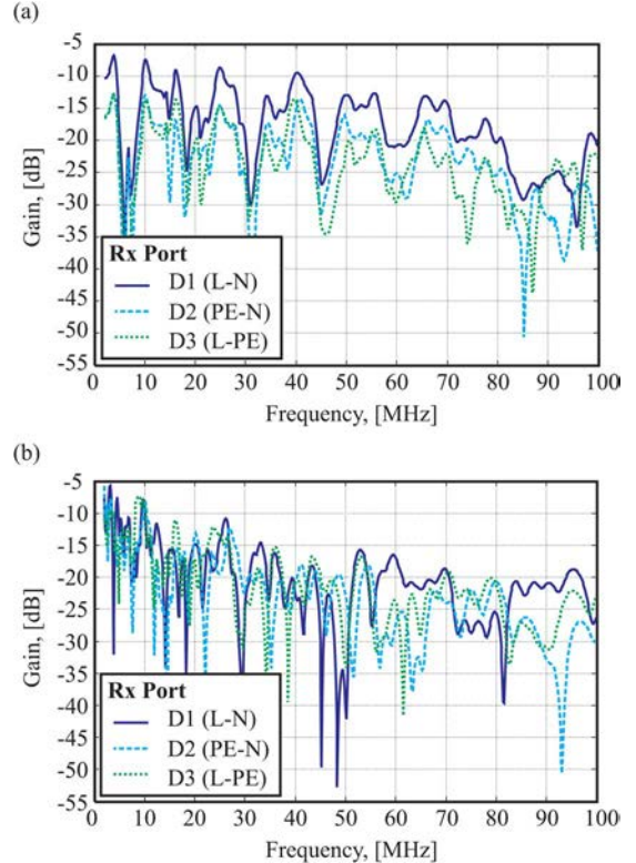
Fig. 4. MIMO PLC CTF examples. (a) CTF measured within an experimental measurement campaign in France [60]. (b) CTF simulated using the MIMO PLC channel model of Hashmat et al. [62]. All results are only shown for tx port D1 (L-N).
