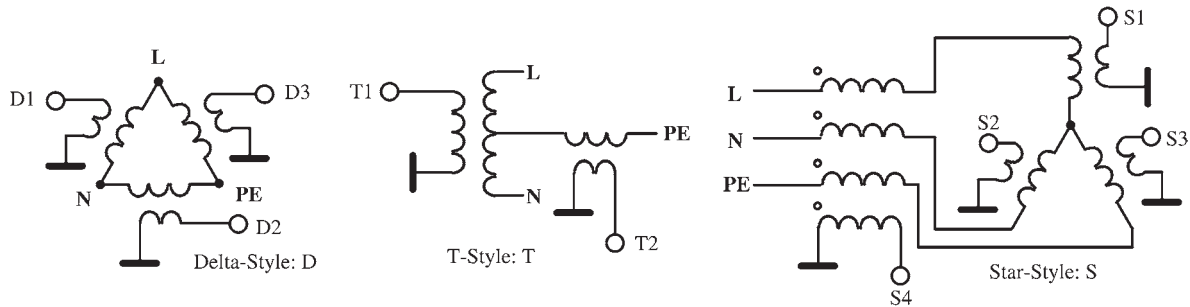
Fig. 1. Inductive MIMO PLC couplers.
