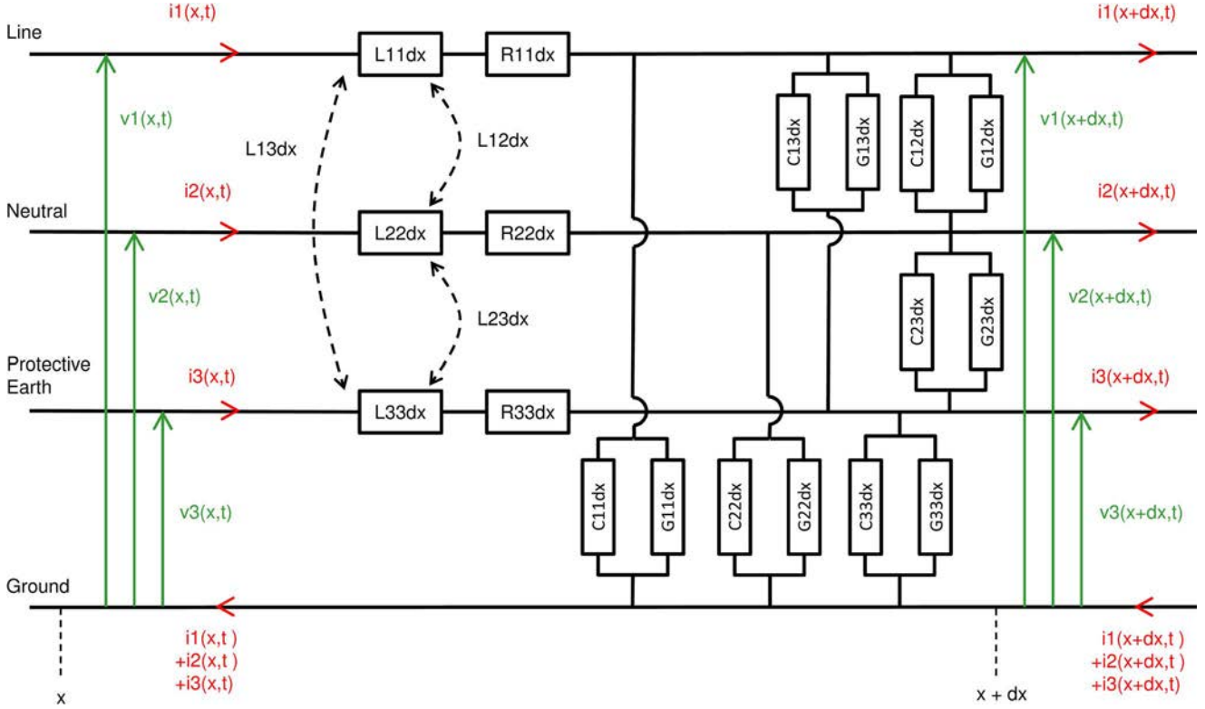
Fig. 3. MTL theory: equivalent circuit of a per-unit length section of a 3-wire transmission line.
