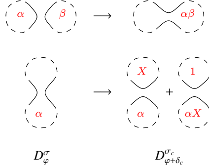
Figure 4: Enhancing rules
