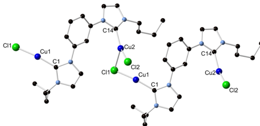
Figure 4. Ball and stick representation of two dinuclear, monomeric units [ImidBuCu 2 Cl 2 ] which are held together by Cl1 and form the polymer chain of 3a in the solid-state. Hydrogen atoms have been omitted for clarity. Selected bond lengths (Å) and angles (°): C1–Cu1 1.882(5), C14–Cu2 1.901(5), Cu1–Cl1 2.1152(14), Cu2–Cl2 2.1835(13), Cu2–Cl1 2.6073(14); C1–Cu1–Cl1 171.34(15), C14–Cu2–Cl2 147.35(15), C14–Cu2–Cl1 113.34(14), Cu1–Cl1–Cu2 89.79(5), Cl1–Cu2–Cl2 98.96(5).
