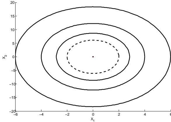
Fig. 1. Contractive ellipsoidal set obtained with Theorem 3 (dashed line) and Theorem 2 (solid line)
