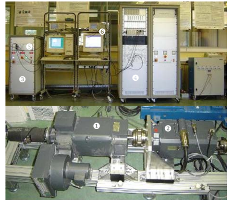
Fig. 13. Components of the G2ELAB test bench, Grenoble, France: ① DC motor, ② PMSG, ③ Power electronics for driving the DC motor, ④ Power electronics for driving the PMSG, ⑤ DSP TMS320F240 implementing DC motor control, ⑥ DSP DS1005 (dSPACE) implementing PMSG-based MCT control.
