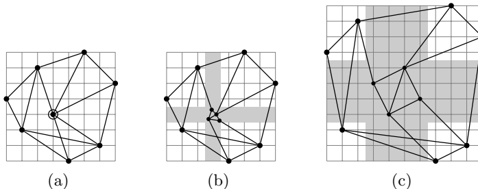
Fig. 1: Expansion of an aggregated node in a rook-drawing of a non-planar graph.
