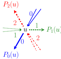
Fig. 5: Orientation around an inner node u in a Schnyder wood.
