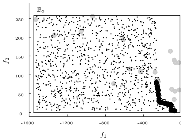
Fig. 8: An illustration, in the objective domain Y_o , of BMOO running on the OSY test problem. The small dots are the particles used for the computation of the expected improvement. They are uniformly distributed on the non-dominated subset of B_o . Dark disks indicate the non-dominated solutions found so far, light gray disks indicate the dominated ones.
