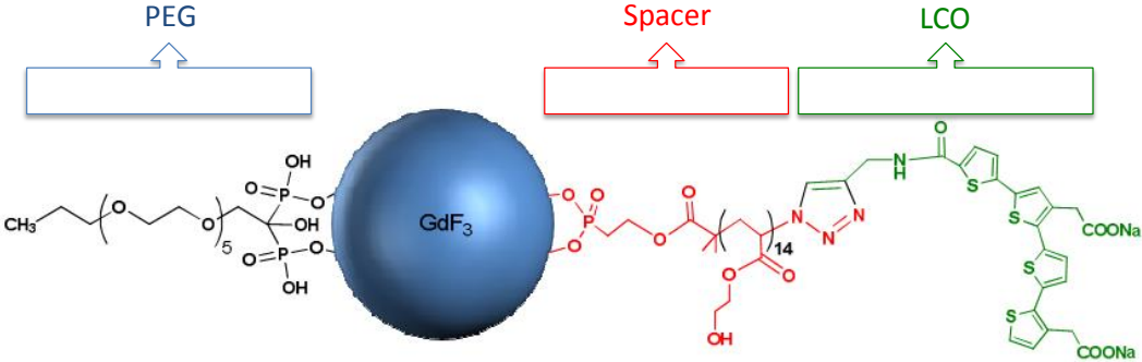
Figure 1. Hybrid nanoparticle 5011.
