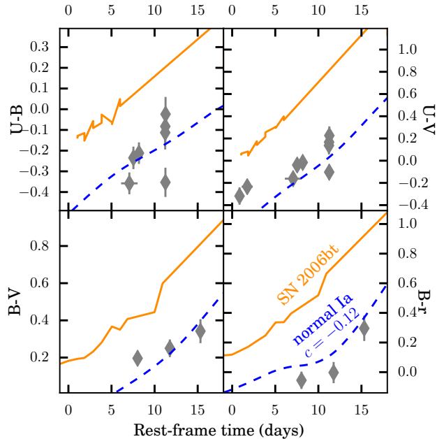
Figure 7. Comparing HFF14Tom observations to the color curves of SN 2006bt and a normal Type Ia SN model. Grey points show the observed colors of SN HFF14Tom, k-corrected to rest-frame UBV r bands. Solid orange lines show the observed color curves for the peculiar Type Ia SN 2006bt. Dashed blue lines show the color curves for a normal Type Ia SN, derived from the SALT2 model with a color parameter c = -0.12 , set to match the best-fit color for SN HFF14Tom.
