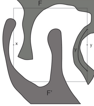
Figure 2: Entanglement point In this example, \{x, y\} \in \mathbf{N}_\varepsilon(F) because the two connected components of P'_{x,y} , in lighter grey, are connected through \gamma \subseteq (F \cap P_{x,y}) . We don't have \{x, y\} \in \mathbf{N}_\varepsilon(F') .
