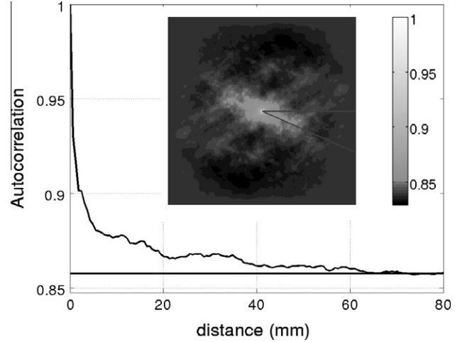
Fig. 9. (map) Covariogram of the equivalent strain presented in Fig. 7c, and (curve) profile of the covariogram for the direction \chi = -32^\circ , corresponding to the largest correlation radius.
