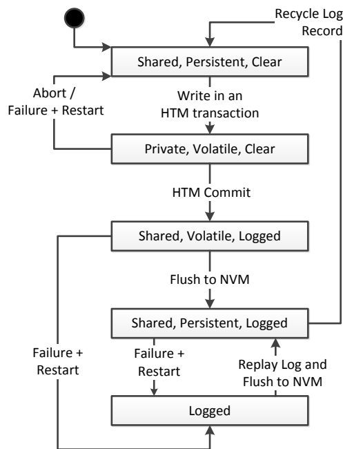
Fig. 1: State machine for a persistent transactional variable
