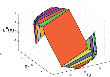
Fig. 7: The piecewise affine controller to recover in Subsection 7.1 with N = 5 .
