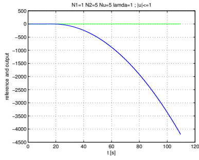
Fig. 5: Reference tracking designed by GPC with N_2 = 5 .
