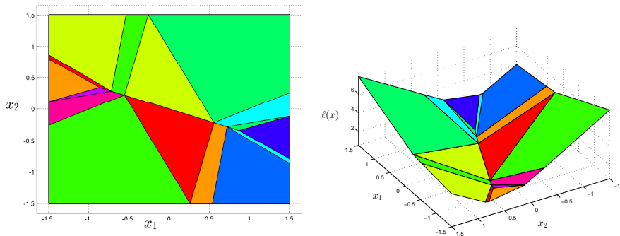
Fig. 11: A subdivision of the polytopic partition in Fig.9 into a convex liftable cell complex.
