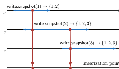
Fig. 2. A write-snapshot execution that is not set-linearizable.
