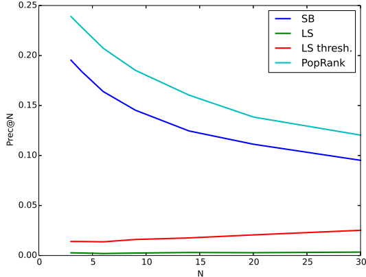
Figure 8: Precision-at- N for N varying in 3-30. The results are averaged over 1,000 users randomly selected among the ML10M database.
