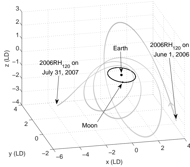
Fig. 2 2006 RH 120 orbit between June 1 st 2006 and July 31 st 2007 in an Earth's centered inertial frame.
