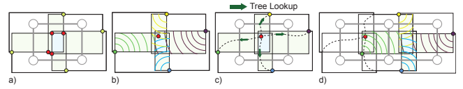
Figure 11: (a) Pairwise seam endpoints closest to a multi-overlap (red) are considered a branching point. (b) This can be determined by finding a minimum point in the multi-overlap with respect to min-path distance from the partner endpoints. (c) After the branching point is found, the new seams are computed by a linear lookup up the partner endpoint's seam tree. (d) To enable parallel computation, each branching point is computed using the initial endpoint location (green) even if it was moved via another branching point calculation (red).
