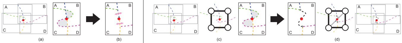
Figure 12: (a) Pairwise seams may produce invalid intersections or crossings in a multi-overlap, which leads to an inconsistent labeling of the domain. The gray area on the top can be given the labels A or B and on the bottom either C or D. (b) Choosing a label is akin to collapsing one seam onto the other. This leads to new image boundaries which were based on energy functions which do not correlate to this new boundary. The top collapse results in a B-C boundary using an A-B seam (C-D seam for the bottom). (c and d) Our technique performs a better collapse where each intersection point is connected to the branching point via a minimal path which corresponds to the proper boundary (B-C). One can think of this as a virtual addition of a new adjacency mesh edge (B-C) at the time of resolution to account for the new boundary.
