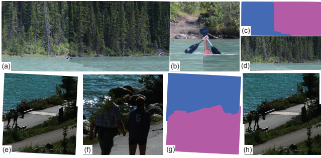
Figure 2: (a, e) Two examples ( Canoe : 6842 x 2853, 2 images and Lake Path : 4459 x 4816, 2 images) of non-desirable, yet exactly optimal seams (unique pairwise overlaps, pixel difference energy). (b, f) A zoom of visual artifacts caused by this optimal seam. (c, g) The pixel labeling. (d, h) The result produced by Adobe Photoshop TM . Images courtesy of City Escapes Nature Photography.
