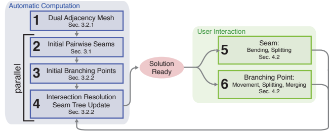
Figure 5: Overview of Panorama Weaving (Sec. 3 and 4). The initial computation is given by Steps 1-4, after which the solution is ready and presented to the user. Interactions, Steps 5 and 6, use the tree update in Step 4 as a background process. Additionally, Step 6 updates the dual adjacency mesh.
