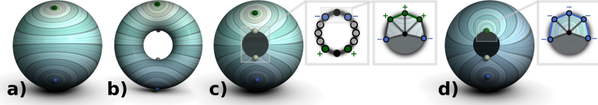
Fig. 3 Non removable critical points: (a) A global minimum and a global maximum have to be maintained for the field not to be constant. (b) 2 g_s saddles cannot be removed. (c),(d) Each boundary component has 2 non-removable global stratified extrema, which turn into non-removable saddles (c) or (possibly) exchangeable extrema (d).
