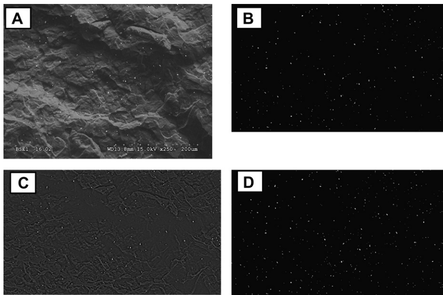
Fig. 2. SEM image of the cryofractured PP_Gd 2 O 3 _1 sample (A). Clipping of Fig. 2-A for a filter power of 37% of its total dynamic (B). Unsharpening of Fig. 2-A with a Gaussian of a 38.4 pixels equivalent \sigma (C). Clipping of Fig. 2-C for a filter power of 20% of its total dynamic (D).
