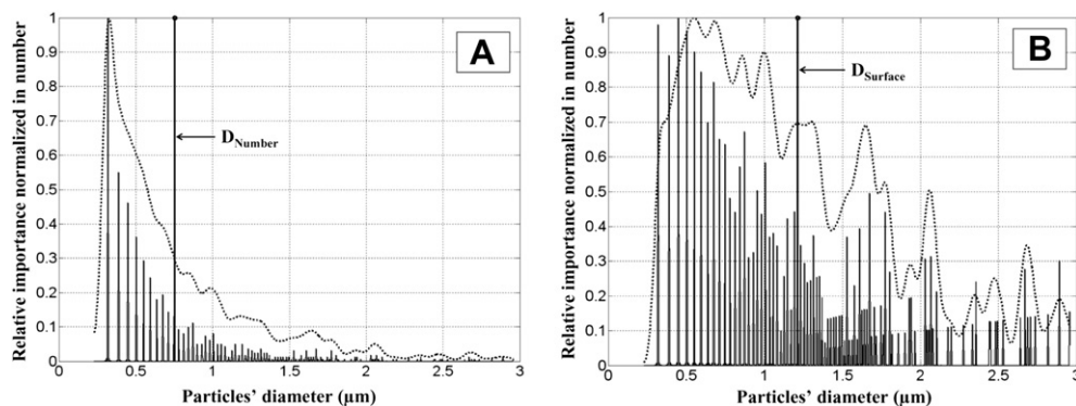
Fig. 5. Number average distribution of particles' diameter for the PP_Gd 2 O 3_1 sample (A) Surface average distribution of particles' diameter for the PP_Gd 2 O 3_1 sample (B).
