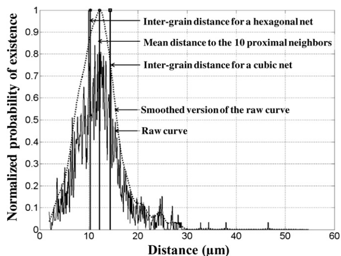
Fig. 3. Curve of spatial dispersion of charges, normalised to the most probable inter-particle distance for the PP_Gd 2 O 3 _1 sample.
