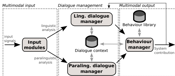
Figure 1: Architecture of the JOKER system
