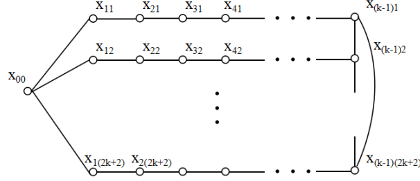
Fig. 2. The ‘‘Cage’’ Graph
