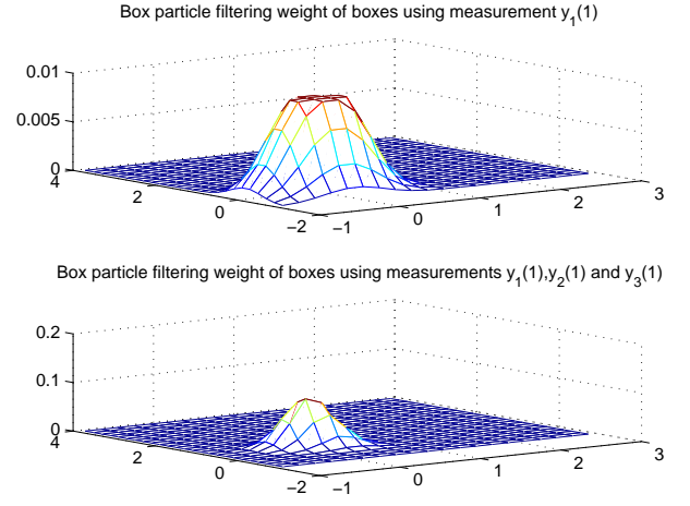
Figure 3: Box weights using measurement y_1(k) (up) and measurements (y_1(k), y_2(k), y_3(k))^T (down)
