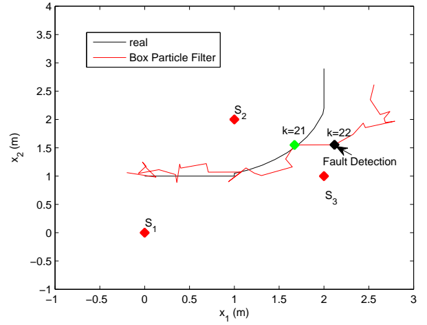
Figure 7: Trajectories in fault scenario
