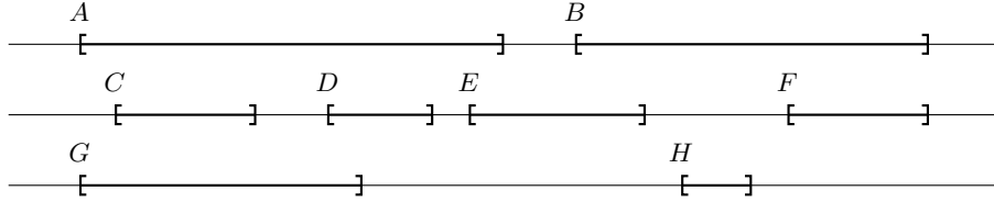
Fig. 2. An example execution involving 3 processes and 8 operations. The point contentions of A , C , D , and G are 3, while E , B , H , and F are 2. The process contention of E is 2, and of B is 3. The interval contentions of A , B , and C are 5, 4, and 3 respectively. The overlapping-interval contention of E is 5.
