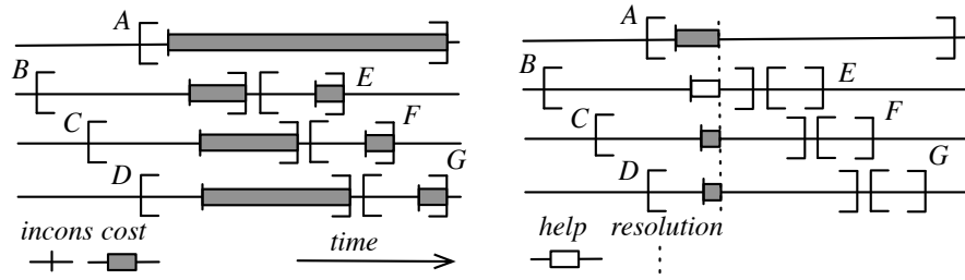
(a) Interval contention without extra help (b) Point contention with extra help
