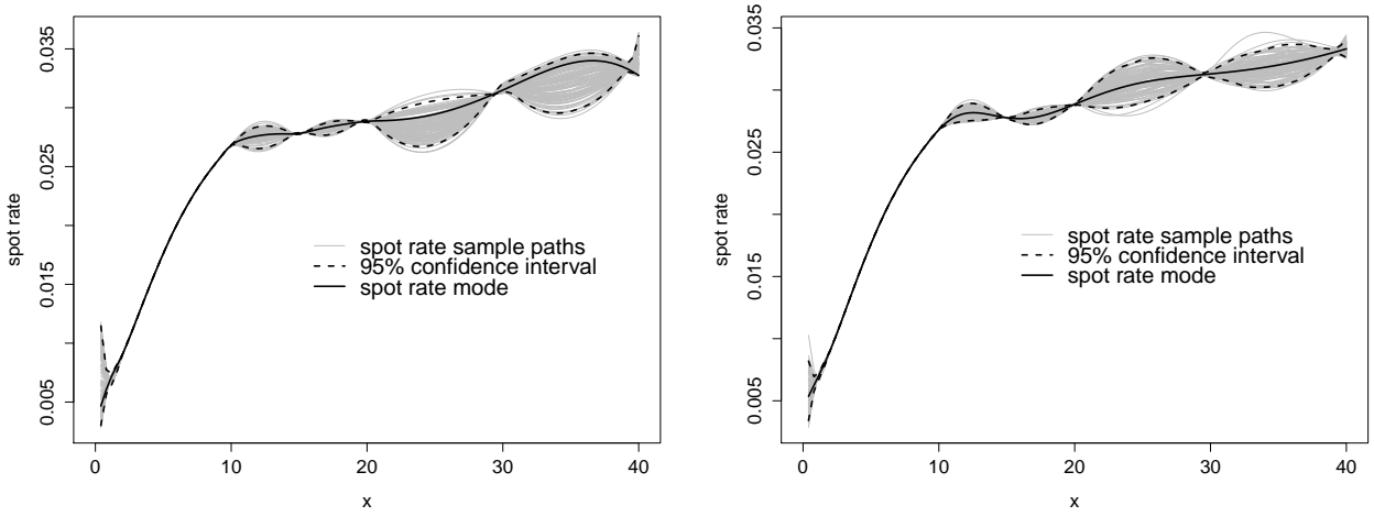
Figure 10: Spot rates obtained from sample paths of Figure 9 with Gaussian covariance function (left) and Matérn 5/2 covariance function (right). Gray lines represent -\frac{1}{x} \log Y^N(x) for each sample path. The black solid line is the most likely spot rate curve -\frac{1}{x} \log M_K^N(x | A, \mathbf{b}) .
