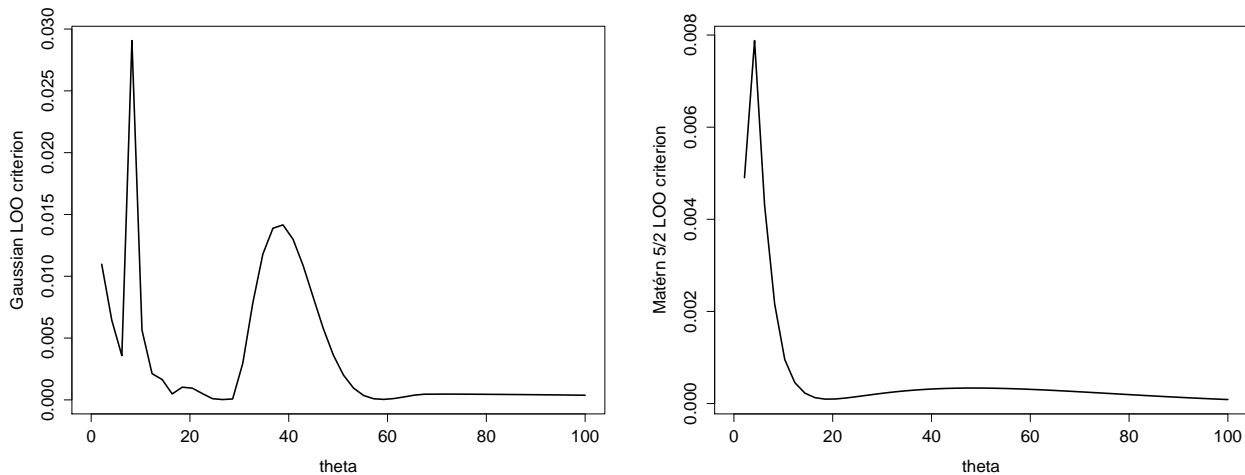
Figure 8: The function to be optimized in LOO criterion (23) using the Gaussian covariance function (left) and the Matérn 5/2 covariance function (right). OIS data on 03/06/2010.
