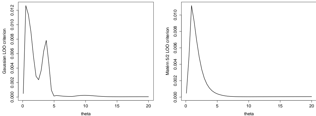
Figure 13: The function to be optimized in the LOO criterion (23) using the Gaussian (left) and the Matérn 5/2 (right) covariance function. CDS quotes as of 11/05/2009.
