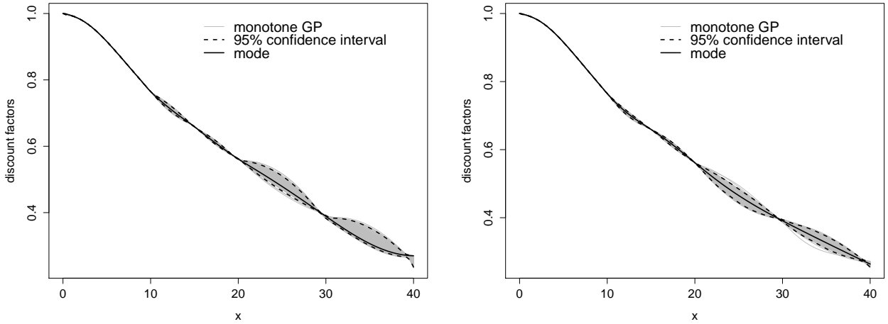
Figure 9: OIS discount factor curves (gray lines) given as simulated paths of a conditional GP with non-increasing constraints using a Gaussian covariance function (left) or a Matérn 5/2 covariance function (right).
