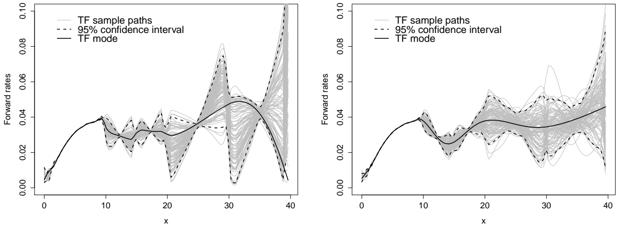
Figure 11: Forward rates obtained from sample paths of Figure 9 with Gaussian covariance function (left) and Matérn 5/2 covariance function (right). Gray lines represent -\frac{d}{dx} \log Y^N(x) for each sample path. The black solid line is the most likely forward rate curve -\frac{d}{dx} \log M_K^N(x | A, \mathbf{b}) .
