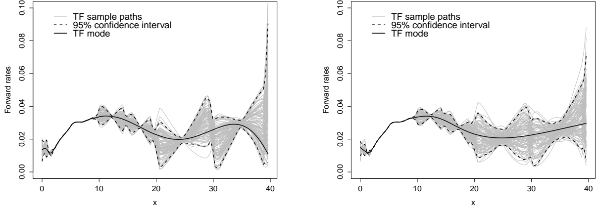
Figure 5: Forward rates obtained from sample paths of Figure 3 with Gaussian covariance function (left) and Matérn 5/2 covariance function (right). Gray lines represent -\frac{d}{dx} \log Y^N(x) for each sample path. The black solid line is the most likely forward rate curve -\frac{d}{dx} \log M_K^N(x | A, \mathbf{b}) .
