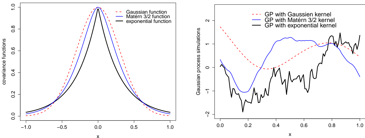
Figure 1: Some Gaussian process covariance functions (left) and associated sample paths (right). The covariance parameters are fixed to (\sigma, \theta) = (1.0, 0.3) .
