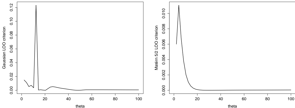
Figure 2: The function to be optimized in the LOO criterion (23) using the Gaussian (left) and the Matérn 5/2 covariance function (right). Swap versus Euribor 6M on 30/12/2011.
