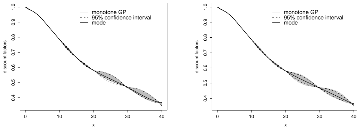
Figure 3: Simulated paths (gray lines) taken from the conditional GP with non-decreasing constraints and market-fit constraints using the Gaussian covariance function (left) and the Matérn 5/2 covariance function (right). Swap vs Euribor 6M market quotes as of 02/06/2010.
