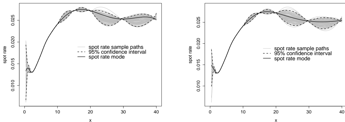
Figure 4: Spot rates obtained from sample paths of Figure 3 with Gaussian covariance function (left) and Matérn 5/2 covariance function (right). Gray lines represent -\frac{1}{x} \log Y^N(x) for each sample path. The black solid line is the most likely spot rate curve -\frac{1}{x} \log M_K^N(x | A, \mathbf{b}) .
