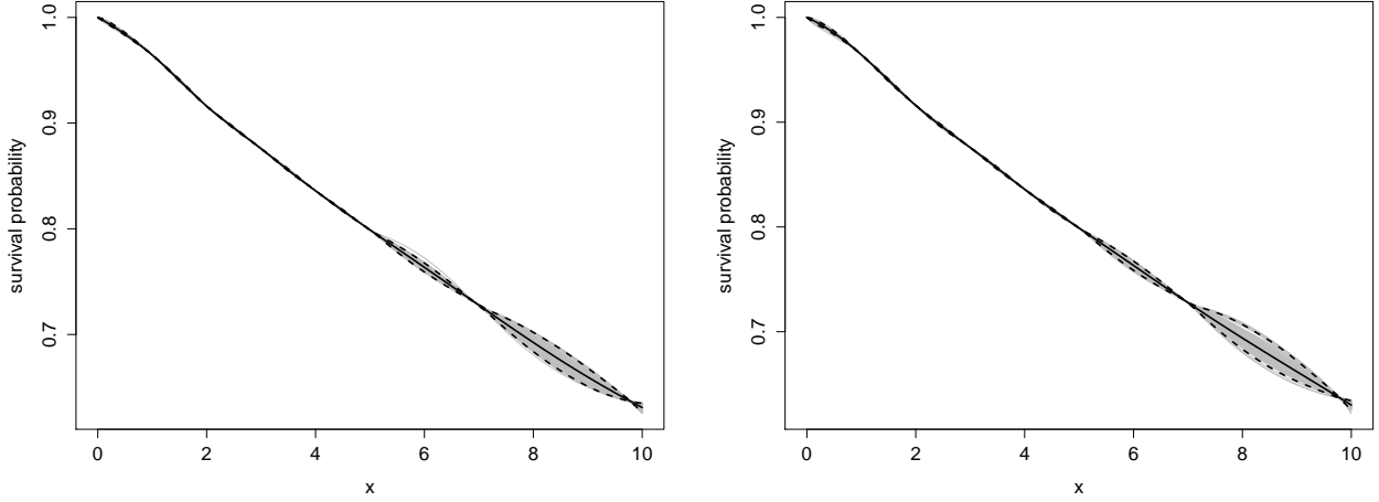
Figure 14: CDS implied survival curves (gray lines) given as simulated paths of a conditional GP with non-increasing constraints using a Gaussian covariance function (left) or a Matérn 5/2 covariance function (right).
