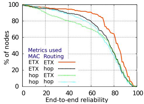
(b) The network has the highest end-to-end reliability when both MAC and routing layers use the same metric ETX (the topology is a cluster-DAG and has 50 nodes)
