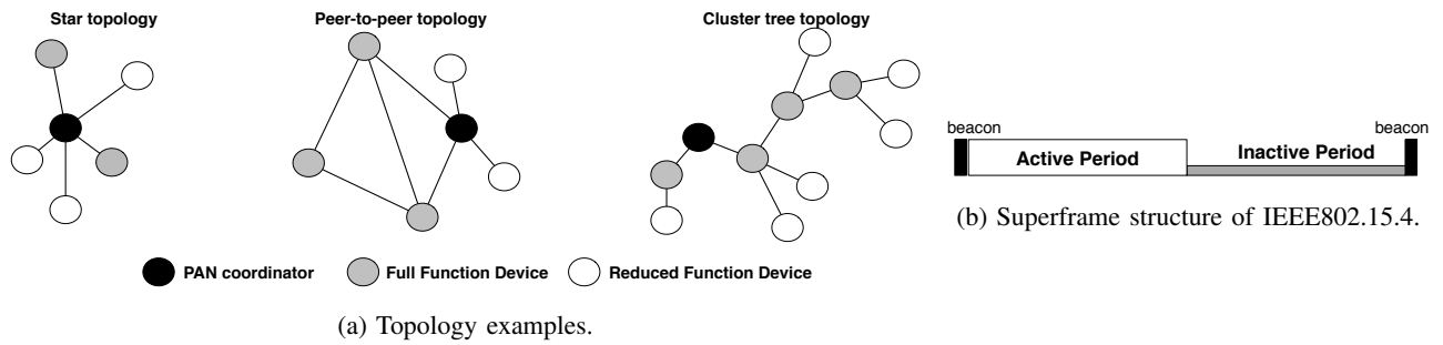
Fig. 1: IEEE802.15.4-2011 concepts.
