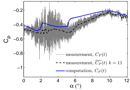
(b) x/c = 0.8
