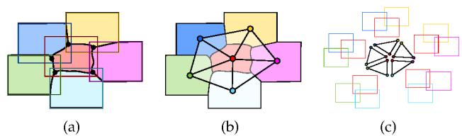
Fig. 5. The seam network for the simple arrangement of the six images shown in (a) is dual to the mesh of (b), where vertices correspond to images, edges to pairwise seams, and faces to branching points. For simple arrangements this adjacency mesh can be constructed as the union of faces corresponding to each overlapping set of images (c).
