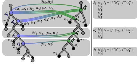
Figure 6: Left: Bipartite graph G between the saddles S^- of \mathcal{T}(f^-) (left) and S^+ of \mathcal{T}(f^+) (right). Each connected component of G yields a unique mandatory n -join saddle (top to bottom: n = 2, 1, 1 ). Right: For each S_k , the list M_k of its mandatory minima and its critical interval I_k is maintained.
