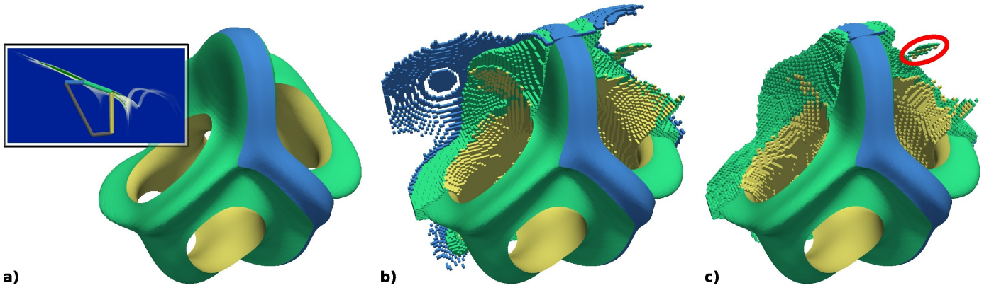
Fig. 9. Clipped view of the tetrahedra returned by our acceleration data-structures for each FSCP edge (matching colors). From left to right: (a) continuous scatter plot, FSCP, output fiber surface, queried tetrahedra with the octree (b, \alpha = 0 ) and the BVH respectively (c, n_T = 1 ).
