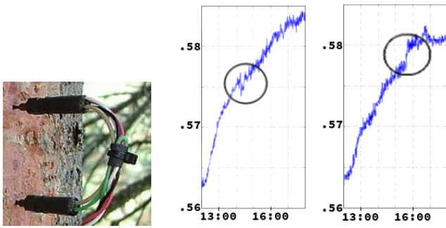
(a) Sap flow sensors: Granier probes are composed of two thermocouple needles. (b) Moving the tree from shadow to sunlight and vice-versa: plots of the output of one Granier Probe (in Volts) in a test tree at LAAS-CNRS lab, on the 8 th and 9 th of April 2015, from 12:00PM to 6:00PM, while the shifting occurred around 3:00PM.
