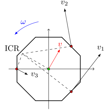
Fig. 9: Instant center of rotation.
