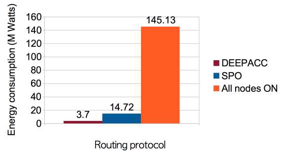
Fig. 3: Energy consumption of 1 layer communication under different protocols
