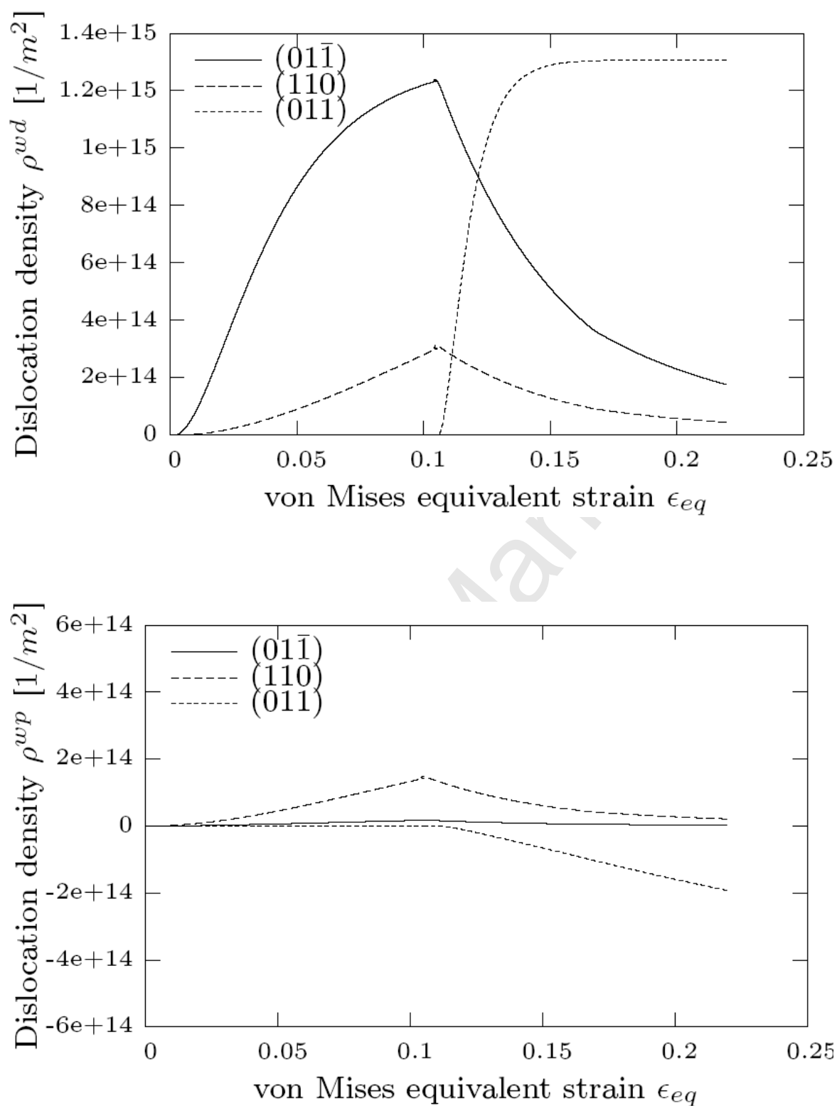
Fig. 10. Evolution of the intensity and polarity of the dislocation sheets in a crystal with initial orientation (32.9, 55.9, 137.4°) during the cross test described in Fig. 9.
