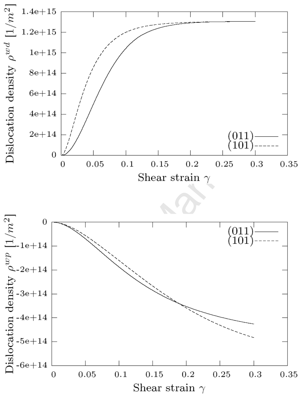
Fig. 5. Evolution of the intensity and polarity of the dislocation sheets in a crystal with initial orientation (-57.5, 138.3, 35.6^\circ) during the simple shear test described in Fig. 2b.
