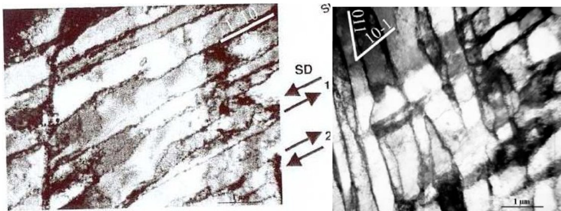
Fig. 6. Longitudinal plane view TEM micrographs (after Peeters et al. [10]): (a) of a (95.6, 124.3, 53.4^\circ) -oriented grain in a specimen after a reverse shear test of -30\%/30\% with SD parallel to RD and SPN parallel to TD, and (b) of a (43.8, 127.8, -42.4^\circ) -oriented grain in a specimen after a reverse shear test of -30\%/30\% with SD parallel to RD and SPN parallel to TD.
