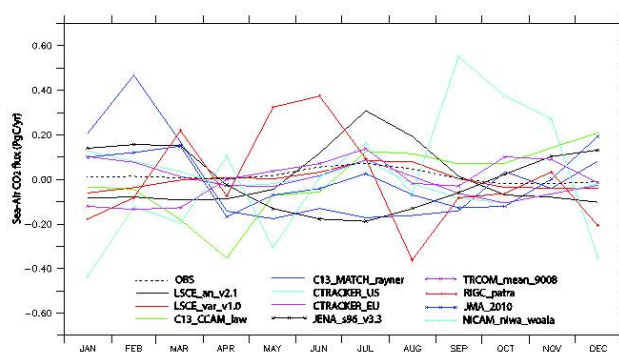
Fig. 10. The seasonal cycle of the sea–air CO 2 flux anomaly for the northern Indian Ocean ( 30^\circ\text{N}\text{--}18^\circ\text{S} ) from atmospheric inversions; overlay on the plot (dashed line) is the observed seasonal cycle.
