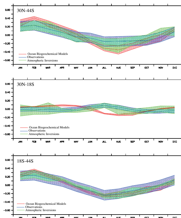
Fig. 6. Seasonal cycle anomaly of the Indian Ocean CO 2 flux ( \text{PgC yr}^{-1} ) from observations, ocean biogeochemical models, and atmospheric inversions for the entire Indian Ocean ( 30^\circ \text{N} – 44^\circ \text{S} upper), northern Indian Ocean ( 30^\circ \text{N} – 18^\circ \text{S} middle) and the southern Indian Ocean ( 18\text{--}44^\circ \text{S} ; lower).
