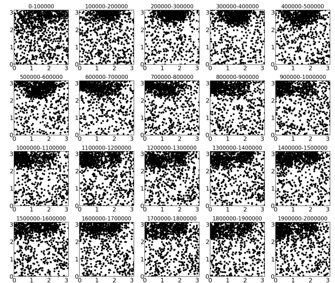
Fig. 5. From top left to bottom right: temporal evolution of the distribution of motor actions executed by the system using the curiosity mechanism in one of the simulations. Each figure represents, in the motor space, the 100000 actions executed by the system during the time window mentioned above the correspond figure.
