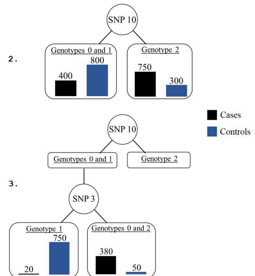
FIGURE 6 | Random forest algorithm. (A) Algorithm of a random forest procedure. (B) An example of the three steps needed to grow one tree.
