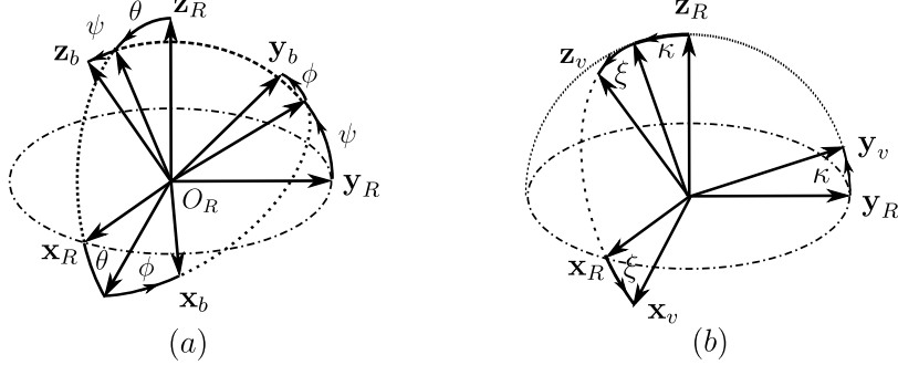
FIGURE 1 – Coordinate systems and relations.
